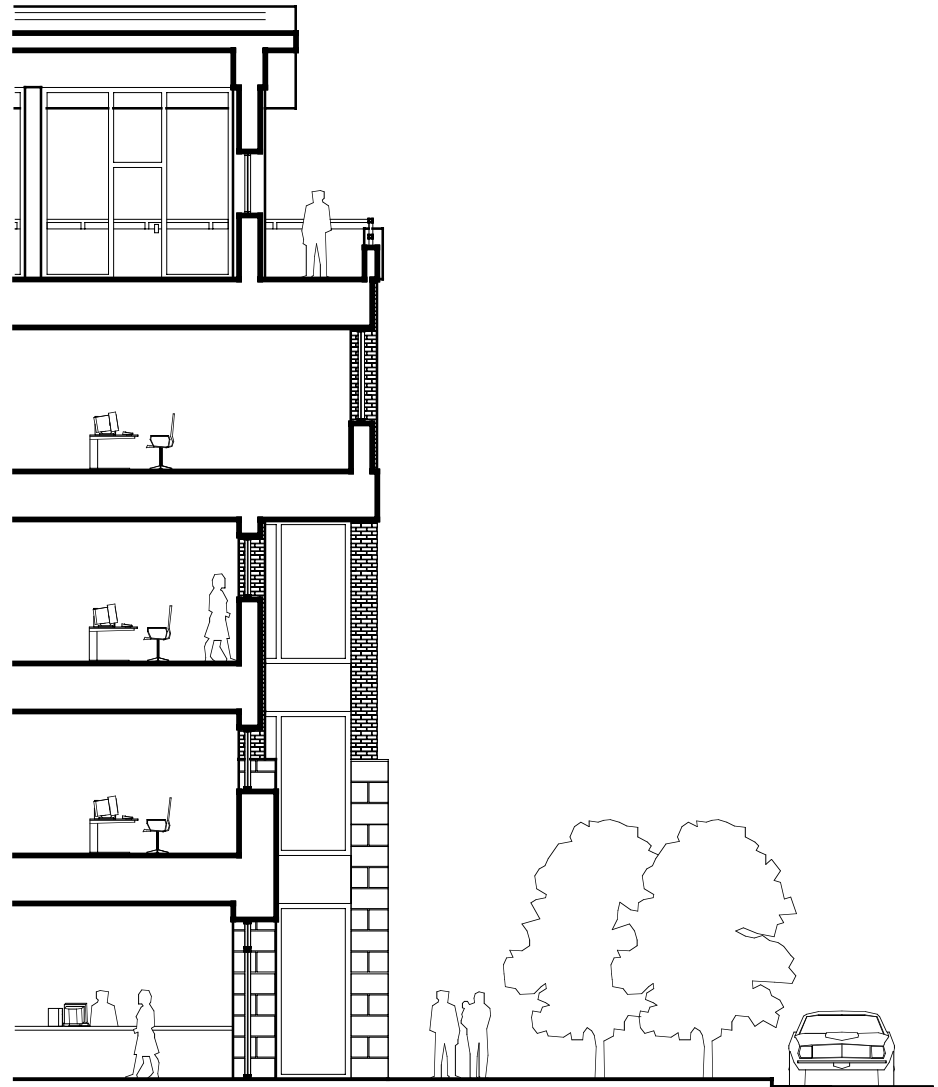
PARTIAL ELEVATION AND SECTION SCALE - 1"=12'
